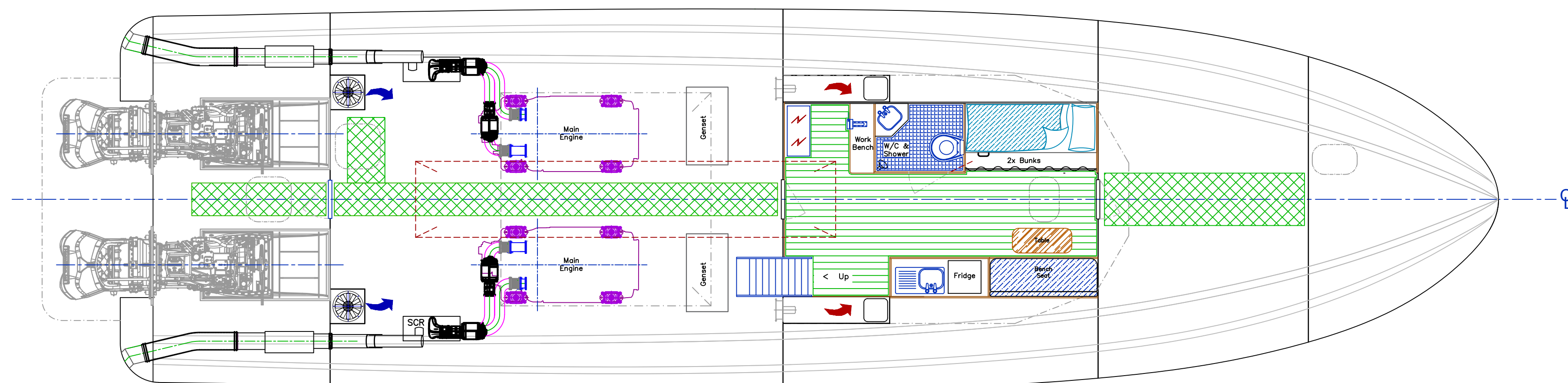
LOWER DECK PLAN
